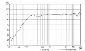
Frequency Response
